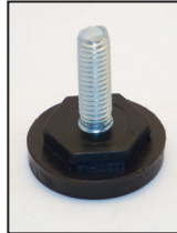
Light Duty, Molded Hex Plastic Base Threaded Glide
